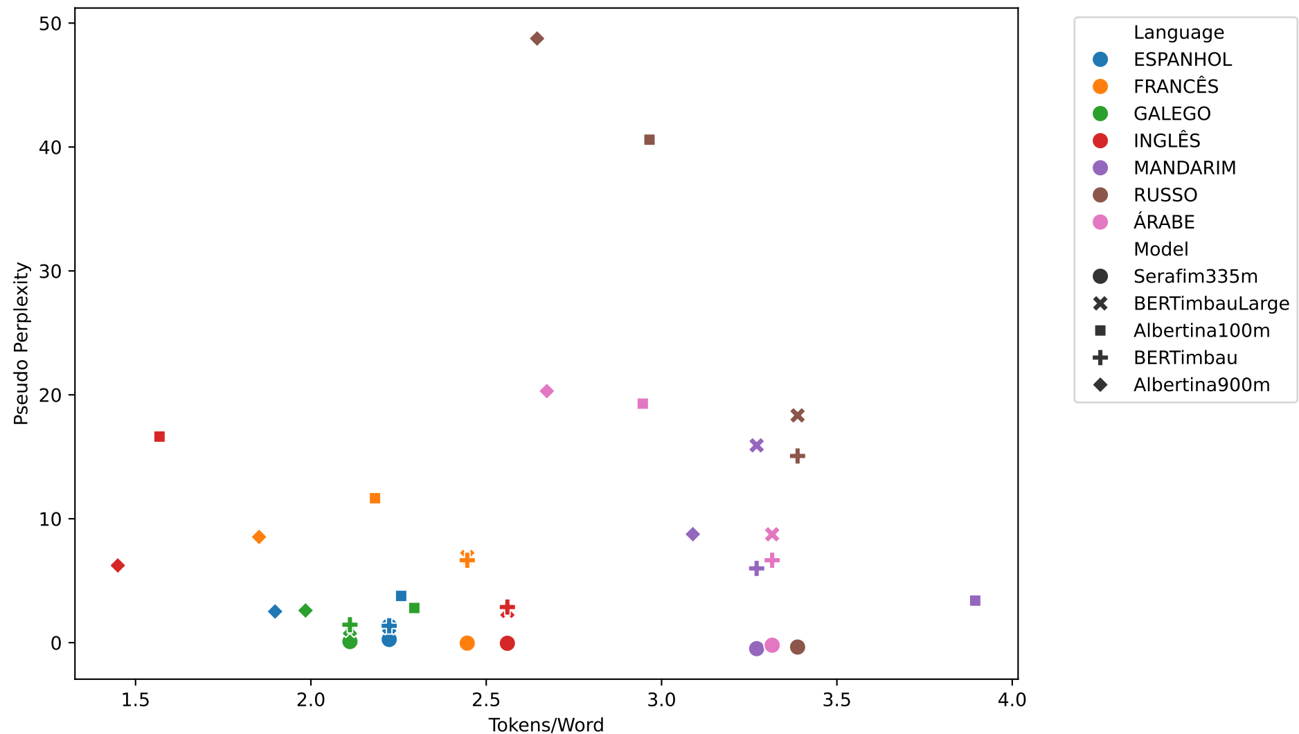
maskedLM - COMPARTILHAR
